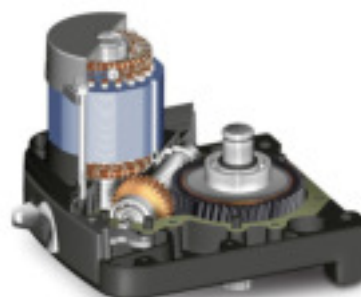
Self locking gearbox and Brushless Motor
